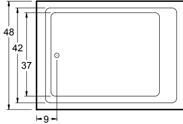
All bathtub dimensions are ± 1/2".
